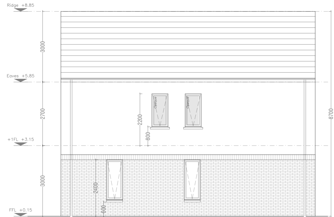
House Type M3 Semi-Detached Side Elevation
